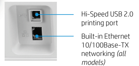
Right side I/O panel closeup
